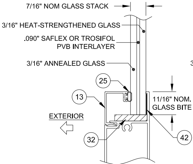
GLASS TYPE 1
