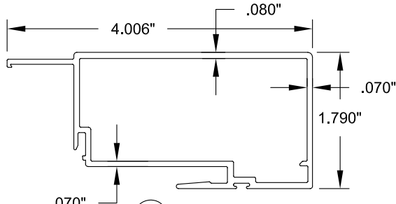
10 INTERIOR INTERLOCK
