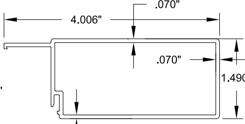
9 VERTICAL STILE
