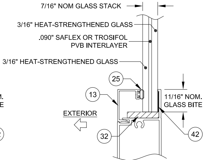
GLASS TYPE 2
