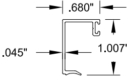
13 BEADING
