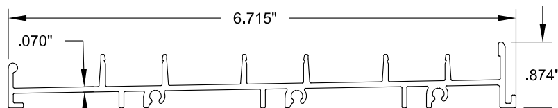
5 3-TRACK SILL
