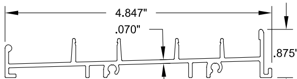
2 2-TRACK SILL
