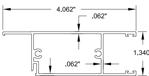
7 HORIZONTAL RAIL
